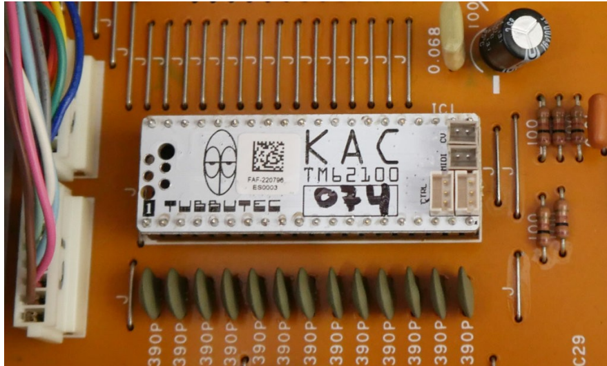
SK30 Mainboard with TM62100
