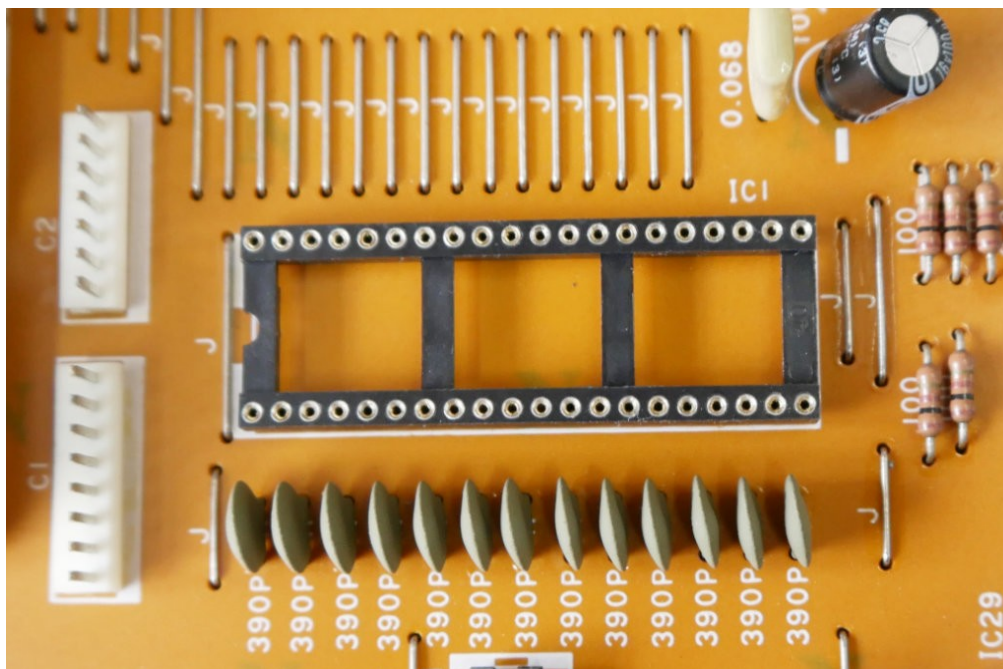
SK30 Mainboard with socket
