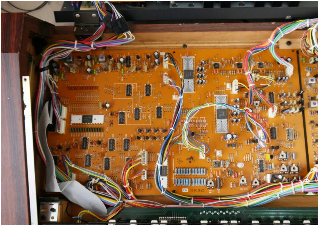
SK30 Mainboard with original KAC
